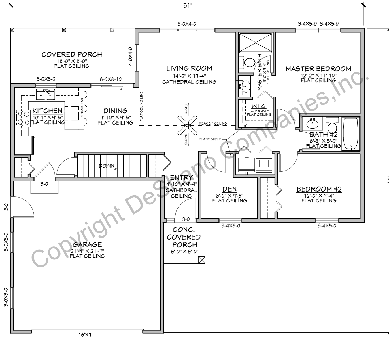
THE EATON SCALE: 1/8" = 1'-0" 1,152 SQ. FT.
