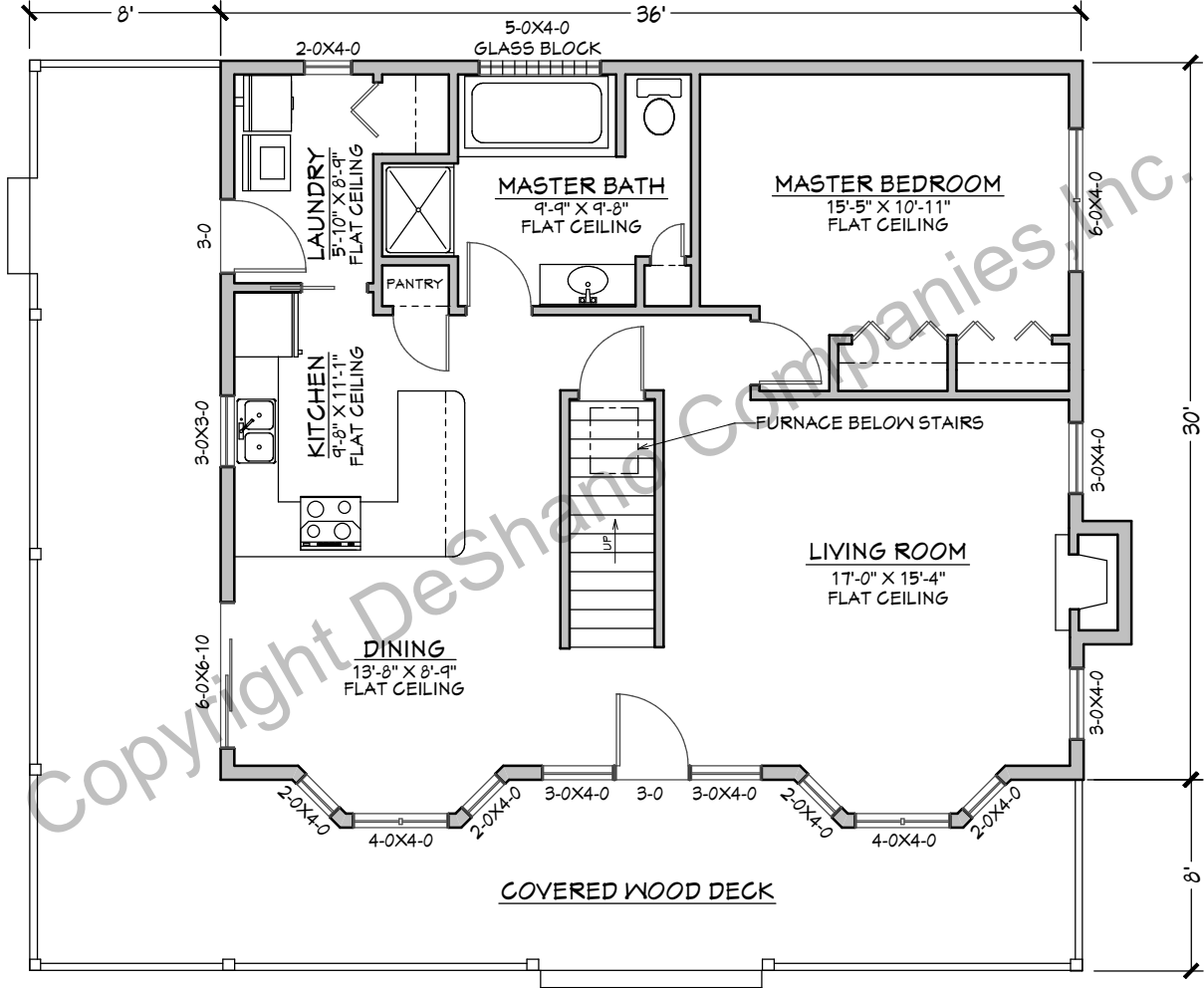
THE SOMERSET SCALE: 1/8" = 1'-0" 1ST FLOOR: 1,113 SQ. FT. 1ST & 2ND FLOOR: 1,876 SQ. FT.
